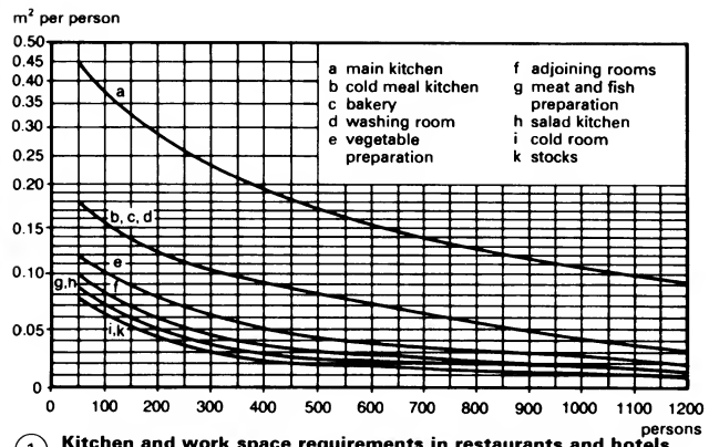
1 Kitchen and work space requirements in restaurants and hotels (a-k = m 2 per person in single room group)
